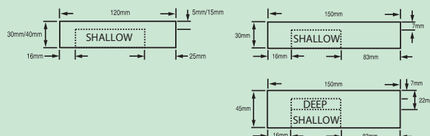
SIZE 2 - SHALLOW BATTERY BOX
