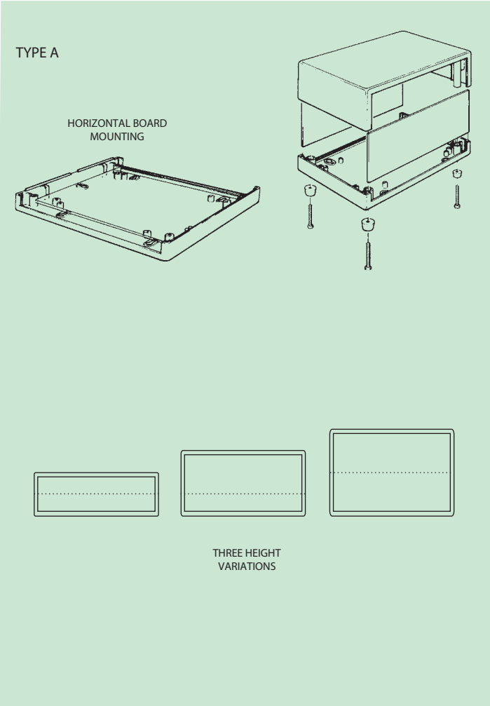
Patina Type A construction (detail)
