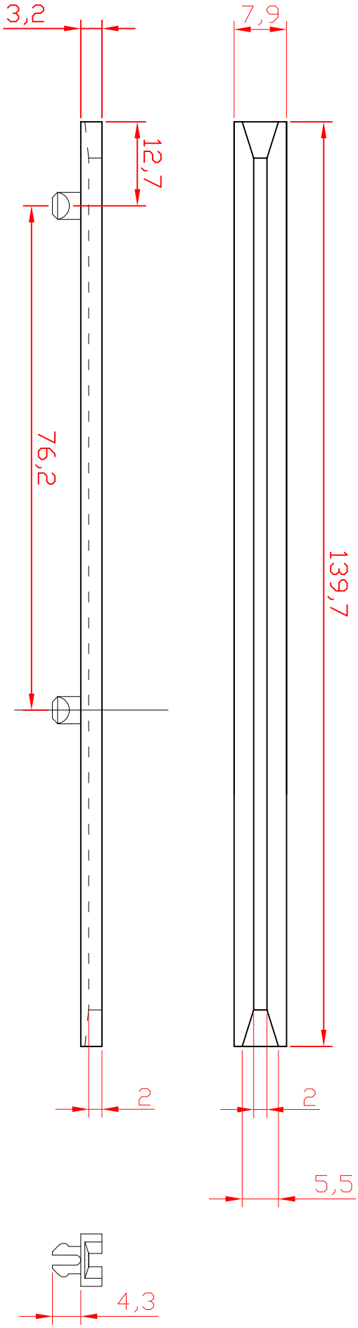
Mounting Hole detail
