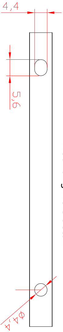
Mounting Hole detail
